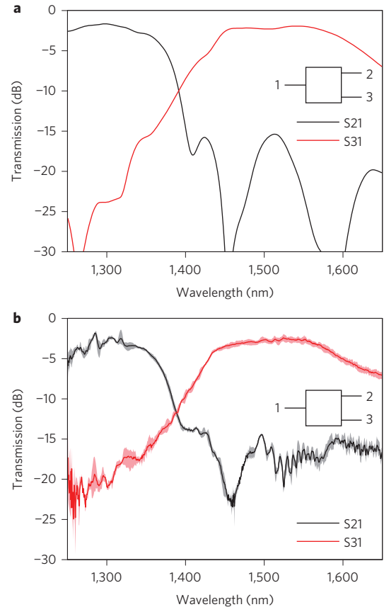
Figure 4 | S-parameters for the device, where S_{ij} is the transmission from port j to port i . a,b , Plots of transmission from input port 1 to output ports 2 and 3: S-parameters simulated using FDTD simulations ( a ); measured S-parameters simulated using three identical devices ( b ). Shaded areas indicate minimum and maximum measured values across all measured devices, and solid lines indicate the average values. The measured devices exhibit relatively low peak insertion losses of -1.8 dB and -2.4 dB in the 1,300 nm and 1,550 nm bands, and broad 3 dB bandwidths of 100 nm and 170 nm, respectively. Crosstalk is less than -11 dB throughout both bands. The insertion losses and crosstalk of the device are somewhat degraded with respect to the simulated values due to fabrication imperfections.
