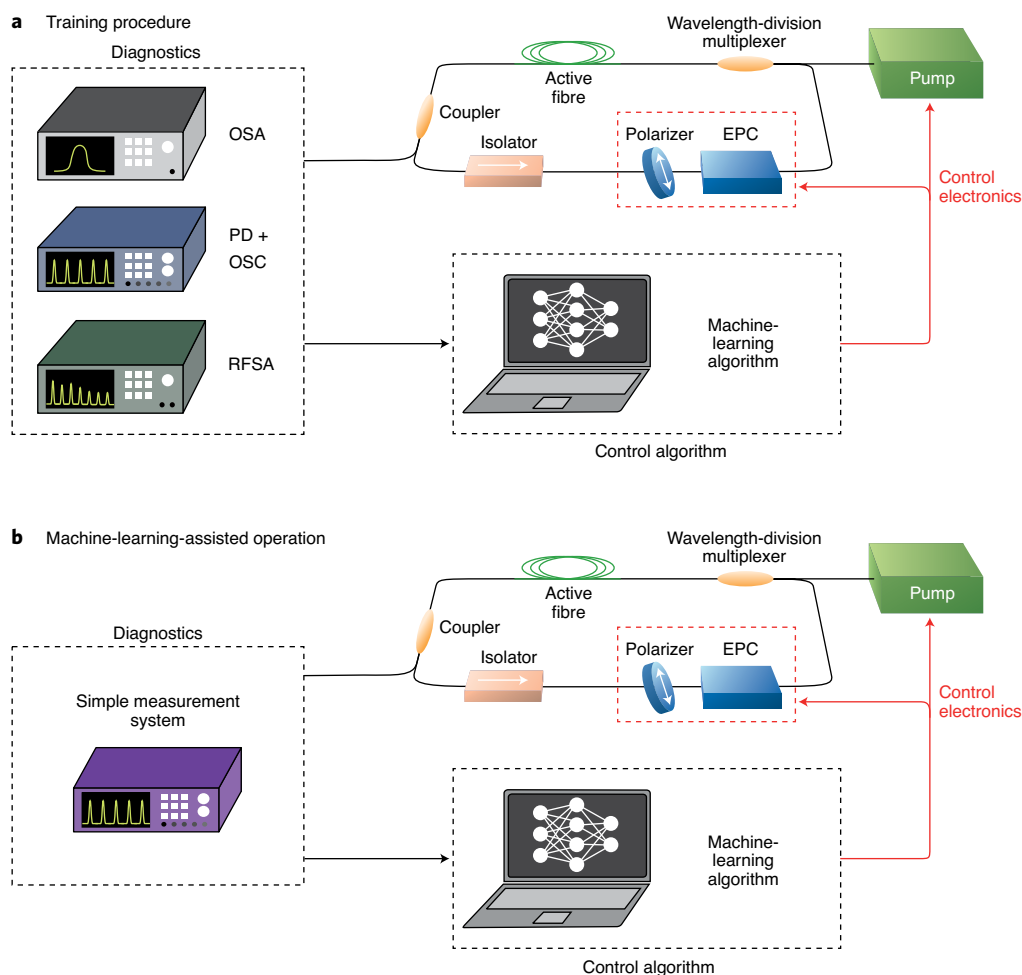
Fig. 2 | Illustration of machine-learning strategies for optimization and self-tuning of ultrafast fibre lasers using control of intracavity elements via a feedback loop and control algorithm. a , Training phase where control electronics acting, for example, on the polarization state (electronic polarization controller (EPC)) sweep the parameter space to map different operating states of the laser to be used as inputs to the control algorithm (Box 1). Guidelines for algorithm and parameter selection are given in Box 2. In the case of a search algorithm, the training phase is not necessary. Output characteristics are measured by diagnostics such as an optical spectrum analyser (OSA), fast photodiode (PD) and oscilloscope (OSC), or radio-frequency spectrum analyser (RFSA), and subsequently used as input to the control algorithm. b , Machine-learning-assisted operation where the laser operation is measured in real time and fed into the control algorithm.
